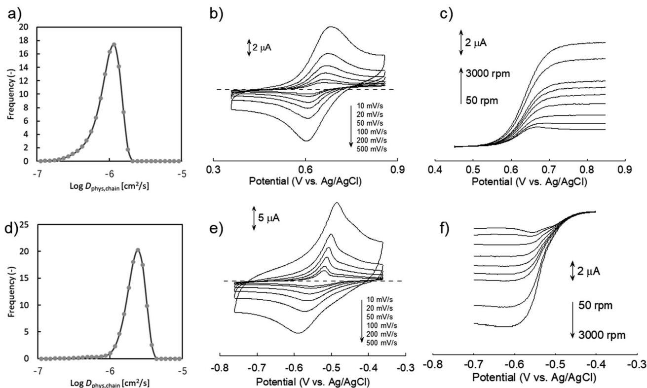
Fig. 3 (a) Distribution of physical diffusion coefficient of P(TMA- r -SBMA) in water, estimated by DLS. (b) Cyclic voltammograms of 2 mM polymer in 0.3 M NaCl aqueous solution with different scan rates. (c) Hydrodynamic voltammograms of 1 mM polymer in the electrolyte, scanned at 10 mV s -1 . The electrode disk was rotated at 50, 100, 200, 400, 600, 1000, 2000, and 3000 rpm. (d) DLS, (e) cyclic voltammograms, and (f) hydrodynamic voltammograms of PVMA aqueous solution, measured under the same conditions.
