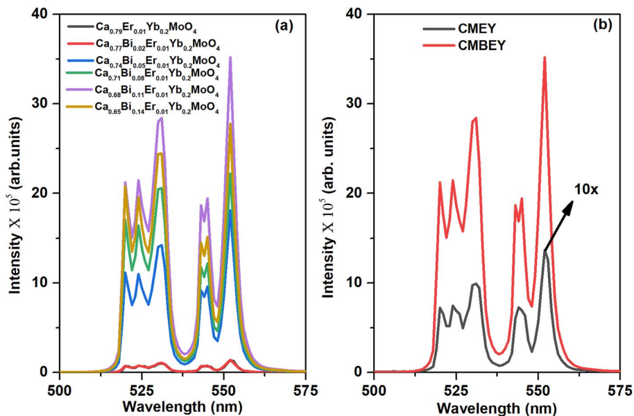
Fig. 5 (a) UC emission of powder samples of \text{Ca}_{0.79-x}\text{Bi}_x\text{Er}_{0.01}\text{Yb}_{0.2}\text{MoO}_4 , with varying Bi concentrations ( x = 0.00, 0.02, 0.05, 0.08, 0.11, and 0.14 ), (b) comparison of the UC emission spectra of CMEY and CMBEY samples both using 980 nm laser as excitation source.
