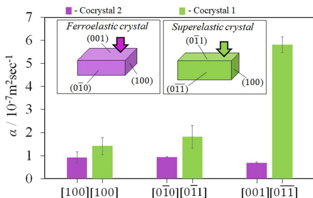
Fig. 5 The obtained thermal diffusivity values of cocrysal 1 (light green colored) and 2 (purple colored) with respect to the longer, wider, and thinner axes, respectively. Arrows indicate the direction of shear stress deformations.
