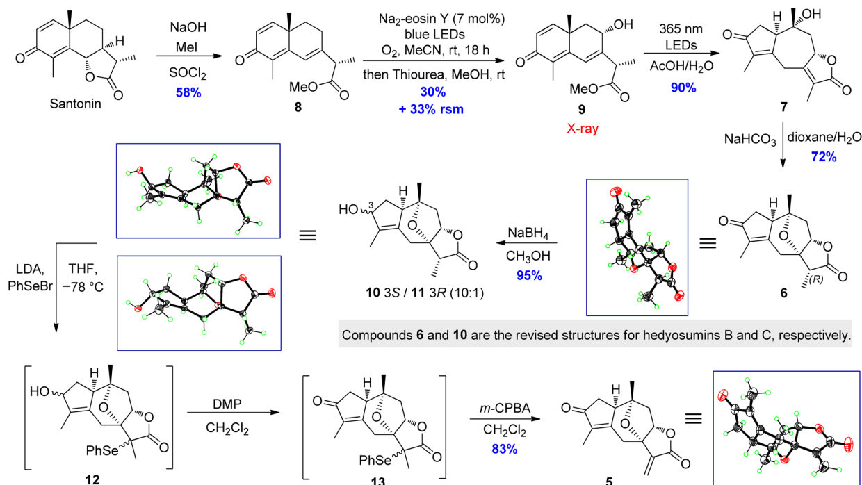
Scheme 3 Synthesis of key intermediate hedyosumin A ( 5 ). LED = light-emitting diode; RSM = recovered starting material; LDA = lithium diisopropylamide; Ph = phenyl; DMP = Dess–Martin periodinane; m -CPBA = meta -chloroperoxybenzoic acid.
