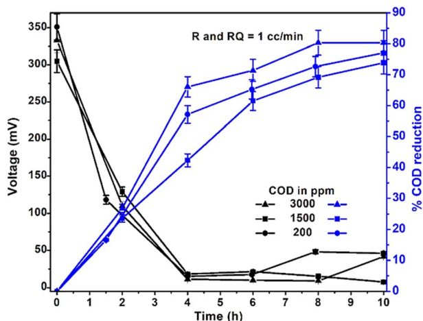
Fig. 5 Operation of the recycle-SCMFC used to treat the industrial wastewater samples ( Q = RQ = 1 \text{ cc min}^{-1} ) at different initial COD values.
