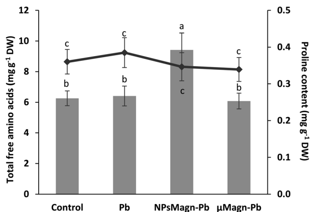
Fig. 4 Total free amino acids ( \text{mg eq leucine g}^{-1} DW) (histogram) and proline content ( \text{mg g}^{-1} DW) (curve) measured in the leaves of sunflower plants after 90 days of growth on control soil or containing Pb, NPsMgn-Pb or \mu Mgn-Pb. Data represent the mean \pm SEM ( n = 6 ). Different letters above the bars indicate significant differences ( p < 0.05 ).
