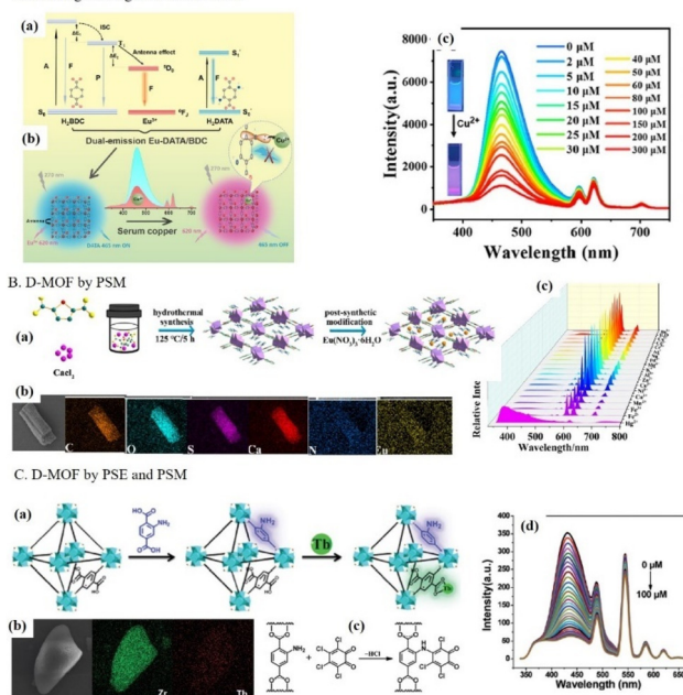
Fig. 13 (A) The design principle and preparation of Eu-DATA/BDC, where \text{H}_2\text{BDC} sensitizes \text{Eu}^{3+} ions to realize the antenna effect emission and DATA maintains its own emission and identifies \text{Cu}^{2+} ions, and the fluorescence spectra of Eu-DATA/BDC in aqueous solutions with \text{Cu}^{2+} ions at different concentrations. Reproduced with permission from ref. 199. Copyright 2022, Elsevier. (B) Eu-Ca-MOF prepared by PSM. (a) The synthesis of Eu-Ca-MOF. (b) The EDX element mapping diagram of Eu-Ca-MOFs and (c) the emission spectra of Eu-Ca-MOFs after treatment with different metal ions. Reproduced with permission from ref. 212. Copyright 2023, Elsevier. (C) The construction of D-MOFs by PSE. (a) and (b) The synthesis procedure, SEM image, and SEM-EDX elemental mapping of \text{Tb@UiO-66-(COOH)}_2\text{NH}_2 . (c) The mechanism of capturing o-TCBQ by \text{atp}^{2-} ligand. (d) The photoluminescence spectra of \text{Tb@UiO-66-(COOH)}_2\text{NH}_2\text{-40} at different concentrations of o-TCBQ. Reproduced with permission from ref. 220. Copyright 2016, the American Chemical Society.
