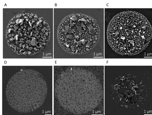
Fig. 2 Representative SEM images of AgNPs spot obtained via SECCM using pipettes with a diameter of \sim 5 \text{ μm} , on a 25-cycle PDA film. The applied potentials were kept constant ( E_1 = -0.4 V and E_2 = -0.2 V vs. Ag/AgCl). (A) [\text{AgNO}_3] = 5.0 \text{ mmol L}^{-1} , t_1 = 0 s, t_2 = 4.0 s; (B) [\text{AgNO}_3] = 5.0 \text{ mmol L}^{-1} , t_1 = 0.5 s, t_2 = 3.5 s; (C) [\text{AgNO}_3] = 5.0 \text{ mmol L}^{-1} , t_1 = 0.5 s, t_2 = 2.5 s; (D) [\text{AgNO}_3] = 0.5 \text{ mmol L}^{-1} , t_1 = 0.5 s, t_2 = 2.5 s; (E) [\text{AgNO}_3] = 0.05 \text{ mmol L}^{-1} , t_1 = 0.5 s, t_2 = 2.5 s; (F) [\text{AgNO}_3] = 5.0 \text{ mmol L}^{-1} , t_1 = 0.5 s, t_2 = 2.5 s, and 50-cycle PDA film.
