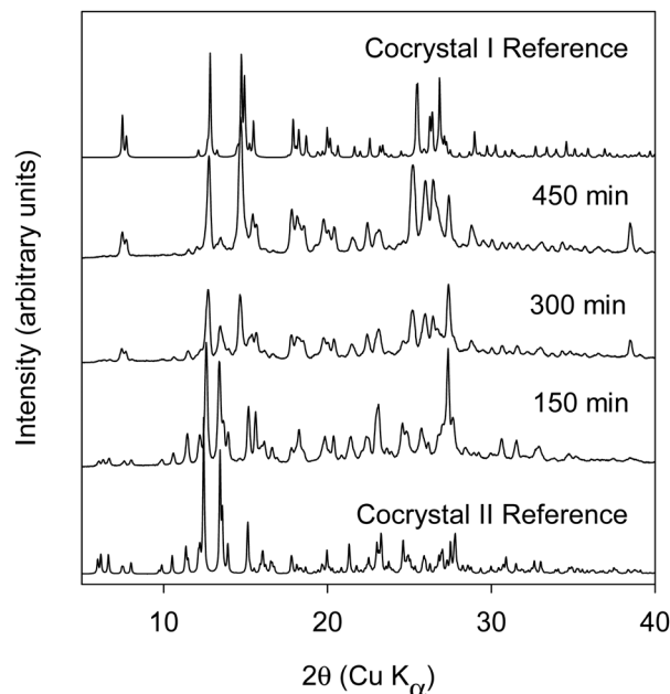
Fig. 4 XRPD data of rBN/BQ at a 1:2 mole ratio subjected to RAM shown in comparison to the reference powder data calculated from the published crystal structures of cocystal I and II. 440 mg of total solids and 1320 mg of zirconia beads were used for the experiment. RAM was done at 75g for all samples.
