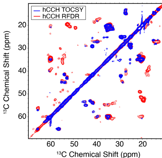
Fig. 5 ^{13}\text{C} - ^{13}\text{C} hCCH spectra of E22G-A \beta_{1-42} amyloid fibrils using TOCSY (red) or RFDR (blue) for carbon homonuclear mixing. Mixing times and other spectral acquisition parameters are tabulated in Table S2 (ESI†).
