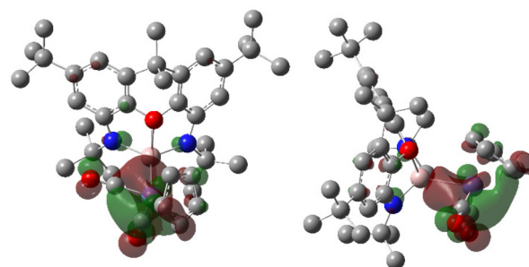
Fig. 3 Molecular orbital (HOMO-2) of the σ(Fe-Al) bond between ( tBu NON)AlFp, showing approximate sigma symmetry along the Al-Fe axis. Hydrogen atoms omitted for clarity, and MO rendered with an iso-value of 0.035 e − Å −3 . Aluminium atom depicted in pale pink and iron atom in purple.
