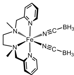
Scheme 2 [\text{Fe}(\text{NCBH}_3)_2(2\text{MeL})] . 85,86
