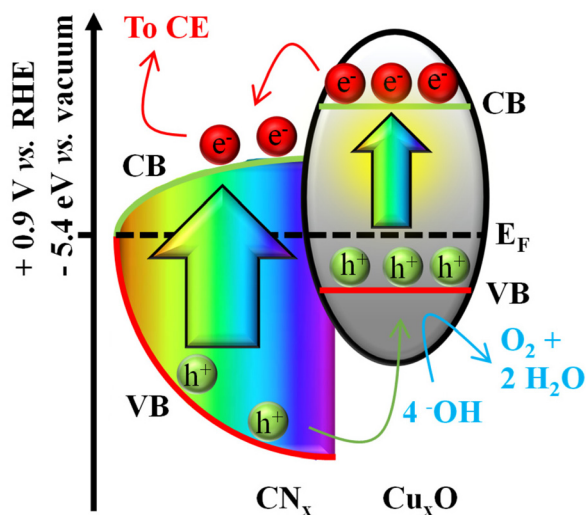
Fig. 11 Approximate band diagram for the \text{CN}_x/\text{Cu}_2\text{O} heterojunction. The positions of VB (valence band) and CB (conduction band) edges for \text{a-CN}_x are represented by red and green curves, respectively. The VB–CB edge separation for \text{CN}_x is proposed considering the E_G values reported in Fig. 2. The Fermi level ( E_F ) position on the vacuum scale was deduced from the work function values reported in Fig. S7.†
