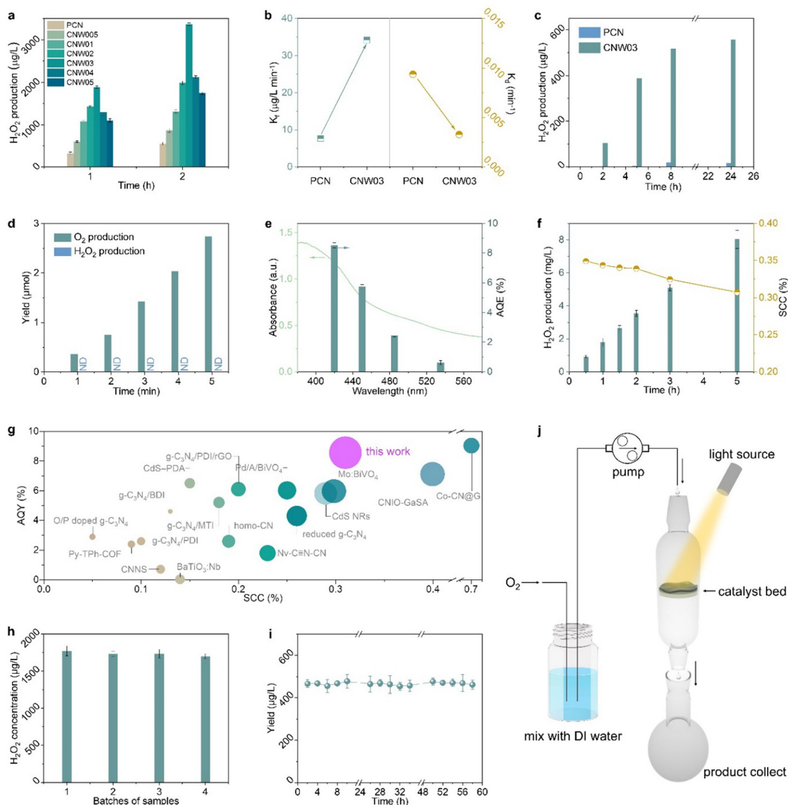
Fig. 3 (a) Photocatalytic H 2 O 2 production on pristine PCN and CNW samples. (b) The corresponding fitted formation rate constants ( K_f ) and decomposition rate constants ( K_d ). (c) Photocatalytic H 2 O 2 production in an oxygen-free environment with an electron acceptor as the reaction trigger under a 1 bar Ar atmosphere. (d) Photocatalytic O 2 evolution and H 2 O 2 production over the CNW03 sample with an electron acceptor under a 0.6 bar Ar atmosphere. (e) AQE of CNW03 as a function of wavelength. (f) SCC efficiency of CNW03 in pure water. (g) Activity comparison of CNW03 with reported state-of-the-art photocatalysts. (h) Cycling stability of the CNW03 catalyst. (i) Long timescale H 2 O 2 production over the CNW03 catalyst in flow mode and (j) the schematic diagram of the corresponding continuous-flow apparatus.
