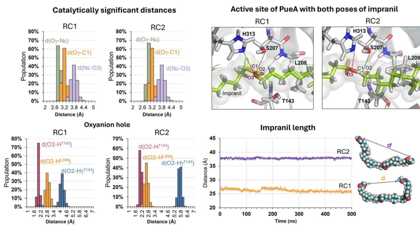
Fig. 3 Analysis of key distances along the 500 ns of free MD simulation of the non-covalent protein:ligand reactants complex with the extended conformation of Impranil when the ester end-group was exposed to the solvent, RC2 . Analysis was done for 2500 structures generated during 500 ns of MD simulation.
