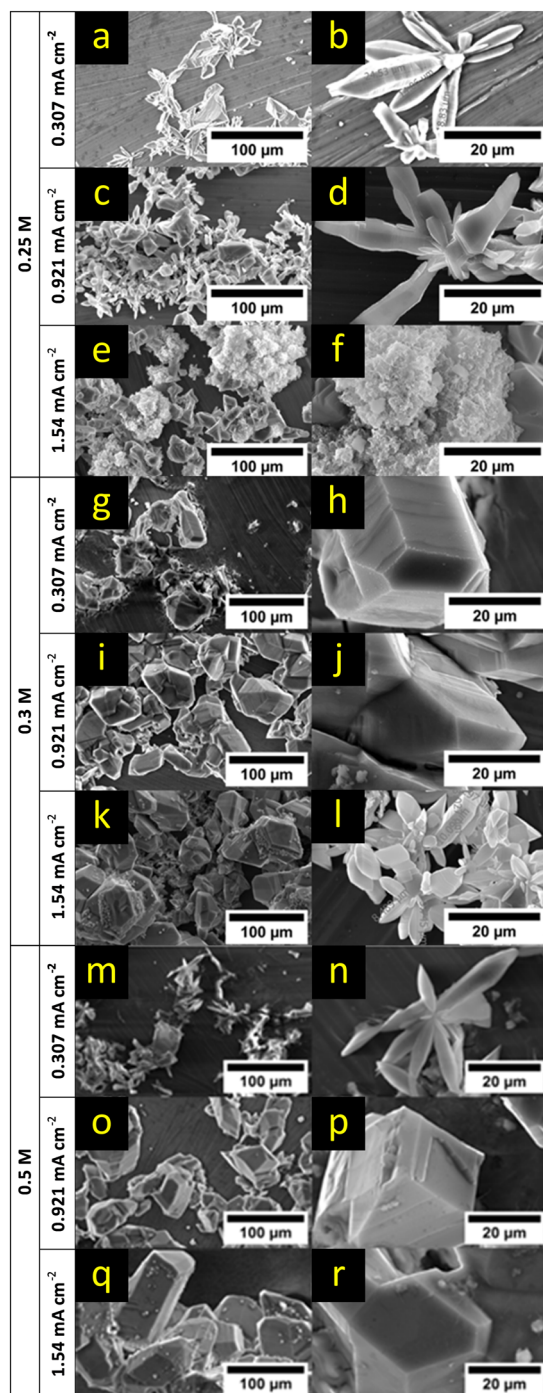
Fig. 4 SEM images after 8 h of magnesium deposition from a 0.25 M (a–f), 0.3 M (g–l) and 0.5 M (m–r) MeMgCl-THF electrolyte solution. The applied current density (rows) can be derived from the subsection of each concentration.
