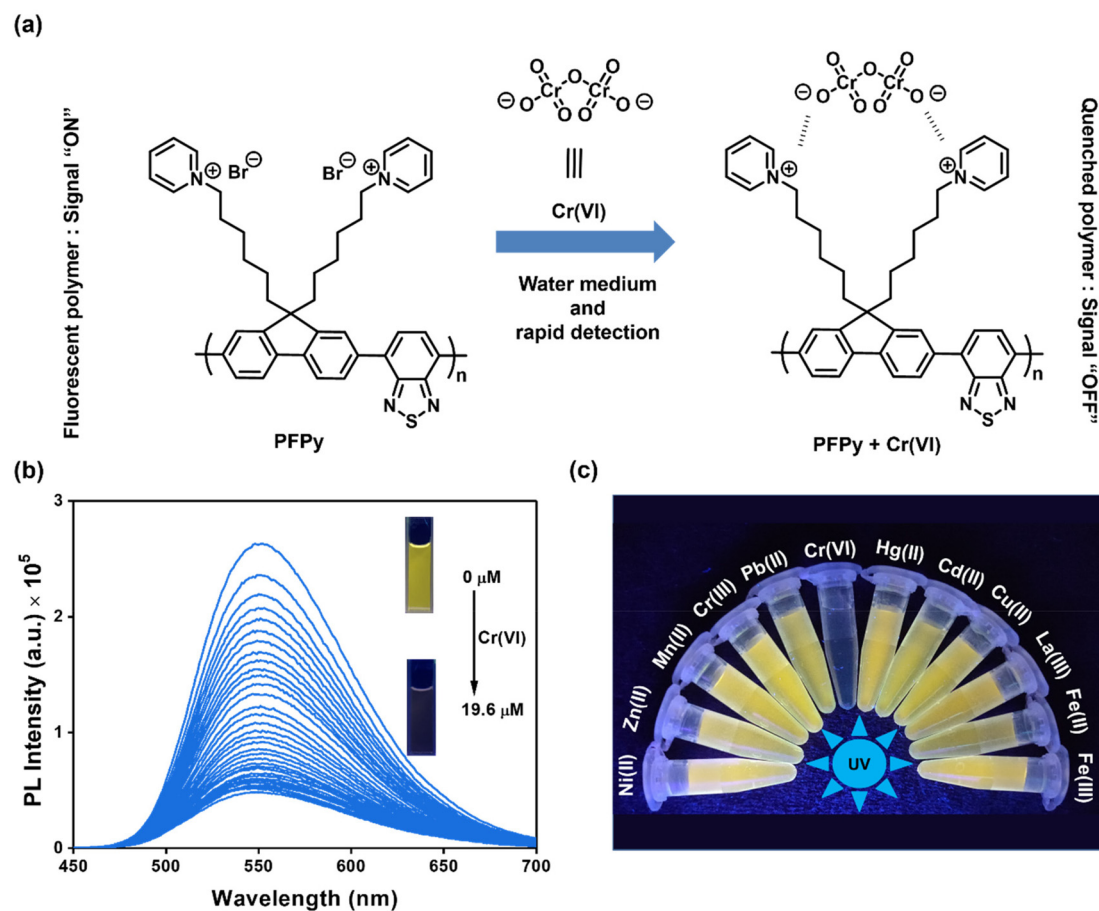
Fig. 1 (a) Chemical structure of PFPy and illustration of \text{Cr(VI)} sensing under an excitation light source; (b) fluorescence spectra of PFPy (6.66 \mu\text{M} ) with an increase in the concentration of \text{Cr(VI)} (inset: images of the PFPy solution before and after addition of \text{Cr(VI)} ); (c) photograph of PFPy solution in the presence of various analytes (20.0 \mu\text{M} ) in water under a UV lamp of 365 nm excitation wavelength.
