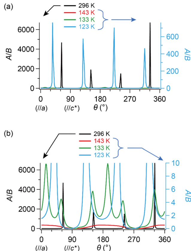
Fig. 8 \theta - and T -dependencies of the ratio of amplitudes in components A and B in eqn (2), A/B , which approximately correlates with the number ratio between SFs and DFs, N_{\text{SF}}/N_{\text{DF}} . The single crystal was rotated around the b -axis, where \theta = 0^\circ corresponds to \mathbf{H} \parallel a -axis. (a) Entire and (b) enlarged view. It should be noted that both curves corresponding to 143 K (red) and 133 K (green) almost overlap with the horizontal axis in (a). Although the unit of angle \theta was radian in the fitting, it is described in degree in this figure.
