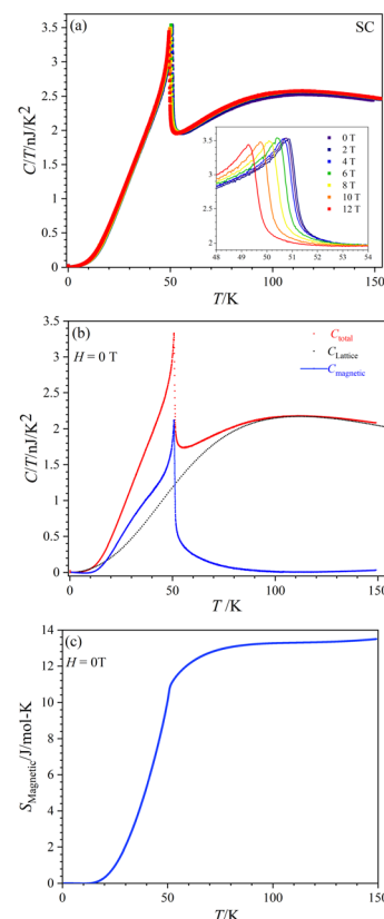
Fig. 8 (a) C/T vs. T curves of CoTeO 4 in the range 0 \leq H \leq 12 T. Inset in (a) represents the zoom view of peak maxima. (b) Magnetic (blue) and lattice (black) contributions of C/T vs. T for H = 0 T. (c) S magnetic vs. T for H = 0 T.
