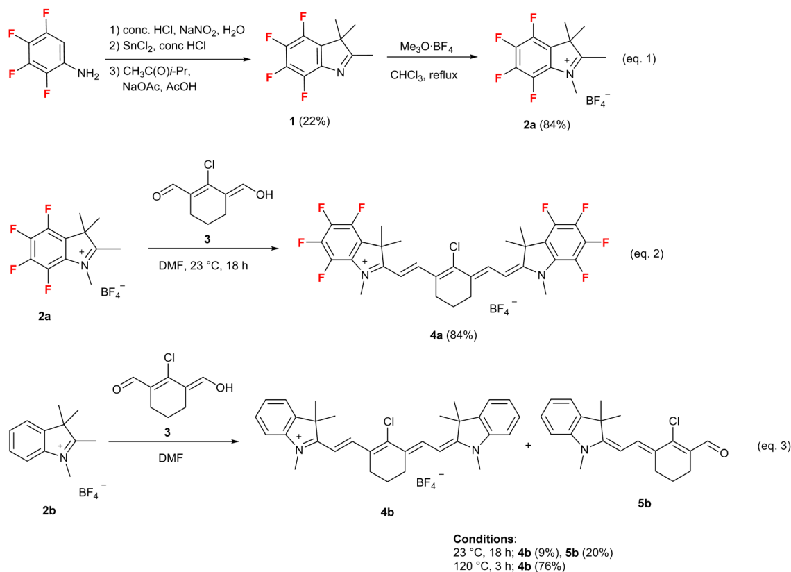
Scheme 1 Preparation of the ring-fluorinated and non-fluorinated HMCDs ( 4a and 4b , respectively).
