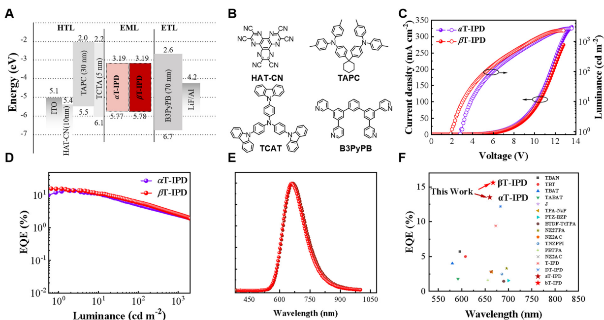
Fig. 4 (A) OLED structure, HOMO and LUMO energy diagram. (B) The material structure used in the functional layer, (C) current density ( J )–voltage ( V )–luminance ( L ), (D) EQE– L curves, and (E) EL spectra of non-doped OLEDs based on \alpha T-IPD and \beta T-IPD. (F) Reported representative hot exciton DR-OLEDs.
