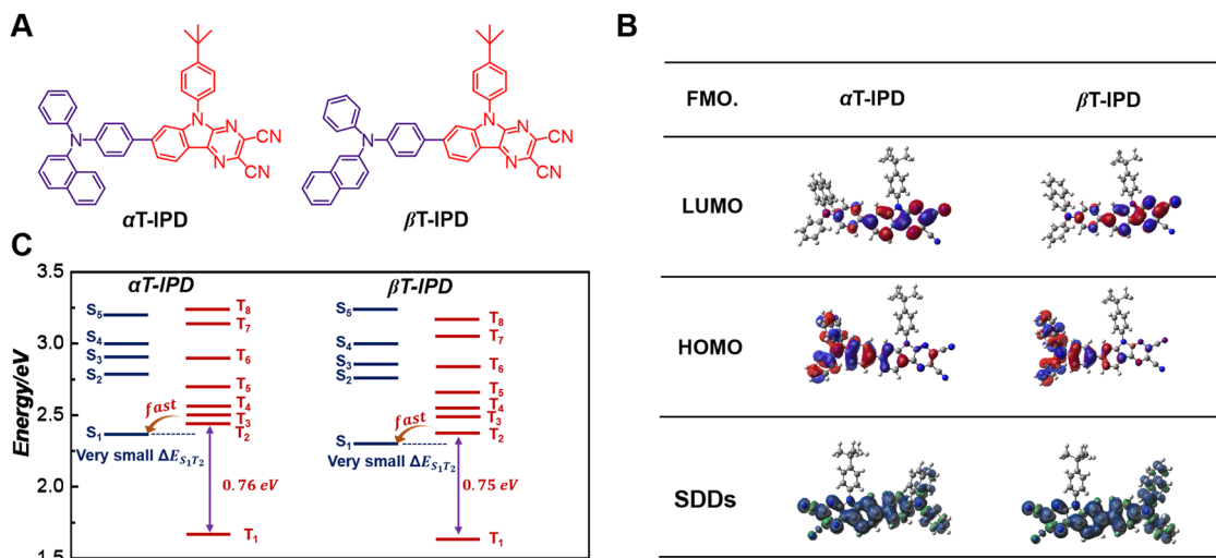
Fig. 1 (A) The chemical structures of \alpha T-IPD and \beta T-IPD. (B) HOMO and LUMO, and T_1 states spin-density distributions (TSDDs) of \alpha T-IPD and \beta T-IPD, respectively. (C) Calculated energy arrangement of singlet states and triplet states of \alpha T-IPD and \beta T-IPD.
