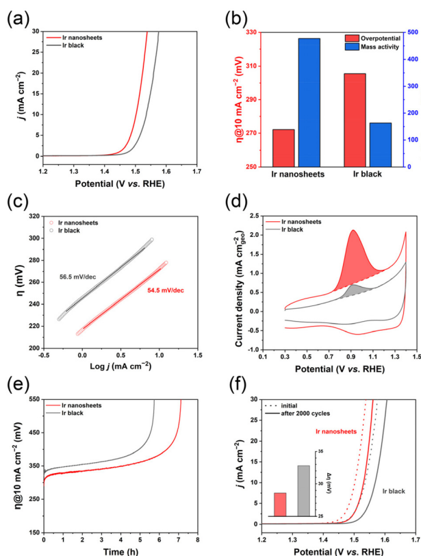
Fig. 4 (a) OER polarization curves of catalysts obtained by LSV in O 2 -saturated 0.5 M H 2 SO 4 at a scan rate of 5 mV s −1 . (b) Overpotentials to drive a current density of 10 mA cm −2 ( \eta@10\text{ mA cm}^{-2} ) and Ir mass activities at 1.53 V vs. RHE of the catalysts. (c) Tafel plots of the catalysts obtained from the polarization curves shown in part (a). (d) CO stripping voltammetry curves of the catalysts obtained in 0.5 M H 2 SO 4 at a scan rate of 20 mV s −1 . (e) Chronopotentiometry curves of the catalysts in O 2 -saturated 0.5 M H 2 SO 4 at a constant current density of 10 mA cm −2 . (f) OER polarization curves of the catalysts in O 2 -saturated 0.5 M H 2 SO 4 at a scan rate of 5 mV s −1 before (dotted lines) and after (solid lines) the ADT. The inset shows the increases in the \eta@10\text{ mA cm}^{-2} of the catalysts after the ADT.
