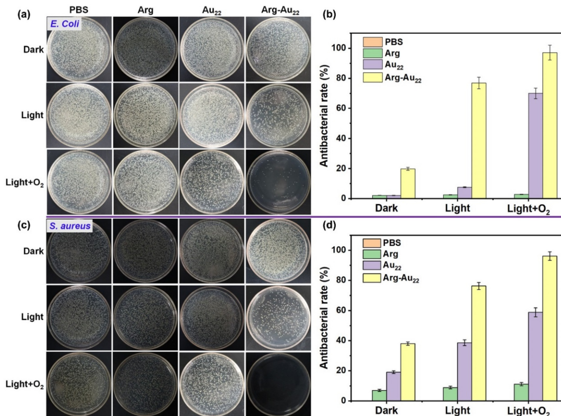
Fig. 2 Bacterial colony growth of (a) E. coli and (c) S. aureus treated with PBS, Arg, Au_{22} NCs and Arg- Au_{22} NCs under dark conditions, visible-light illumination in air, and visible-light illumination with bubbling O_2 . Bactericidal activities of different samples against (b) E. coli and (d) S. aureus .
