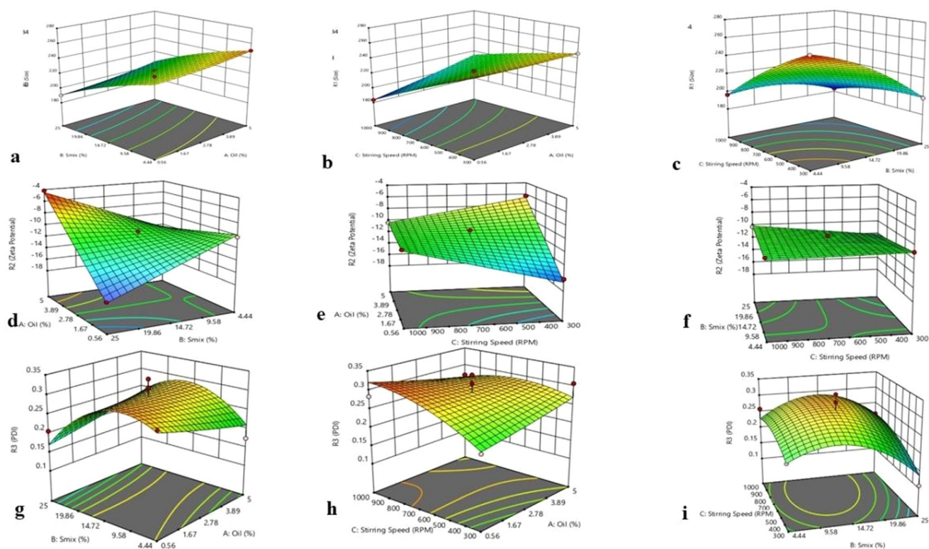
Fig. 3 The 3D response surface illustrating the interaction effect of independent variables, such as the oil concentration, S_{mix} , and stirring speed on the (a–c) particle size, (d–f) zeta potential, and (g–i) PDI.
