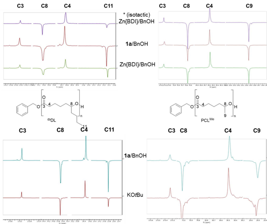
Fig. 1 Zoomed regions of the ^{13}\text{C}\{^1\text{H}\} NMR spectra (100 MHz, \text{CDCl}_3 (top) and (\text{CD}_3)_2\text{CO} (bottom), 25 °C) of \text{PCL}^{n\text{Bu}} (left) and \text{PCL}^{\text{Me}} (right) homopolymers prepared by the ROP of \text{rac-CL}^{\text{Me}} and \text{rac-CL}^{n\text{Bu}} , respectively, except for the spectra labeled (*), prepared from enantiopure ( S )- \text{CL}^{\text{Me}} and ( R )- \text{CL}^{n\text{Bu}} , respectively, mediated by the \text{Zn}\{\text{BDI}^{\text{DIPP}}\}/\text{BnOH} , \text{Y}\{\text{ON}(\text{N})\text{O}^{t\text{Bu}2}\} ( 1a )/ \text{BnOH} and \text{KOtBu} catalytic systems (Table S1,† entries 1–4). The low intensity signals observed are assigned to the terminal repeating units in these low molar mass polymers.
