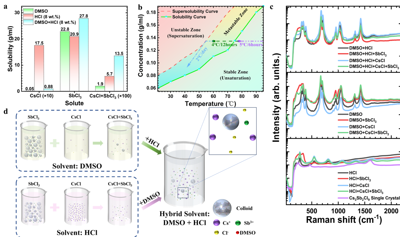
Fig. 1 Dissolution conditions in different solvents. (a) Solubilities of CsCl, SbCl 3 , CsCl and SbCl 3 mixed powders in different solvents at 75 °C. For a clearer presentation, the solubility values of CsCl are multiplied by 10, and that of CsCl + SbCl 3 mixed powders are multiplied by 100. (b) Solubility curve and concentration at different temperatures. (c) Raman spectra of the upper clear layers of the well-stirred solutions prepared by CsCl, SbCl 3 , and CsCl and SbCl 3 mixed powders. Black: pure solvent, red: SbCl 3 solution, blue: CsCl solution, green: solution prepared using CsCl and SbCl 3 mixed powders. (d) Schematic diagram of the precursor solution state.
