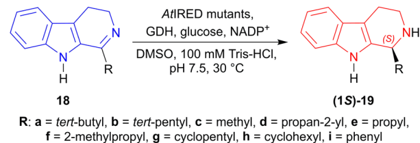
Scheme 43 Reduction of 1-substituted-DH \beta C with AtIRED mutants.
