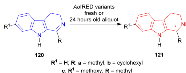
Scheme 37 Reduction of 1-substituted-DH \beta C with fresh or 24 hours old aliquot of AoIRED variants.
