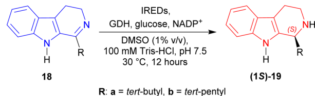
Scheme 42 Reduction of 1-substituted-DH \beta C with IRED-G, IRED-I–IRED-M.
