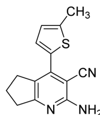
2-Amino-4-(5-methylthiophen-2-yl)-6,7-dihydro-5H-cyclopenta[b]pyridine-3-carbonitrile
