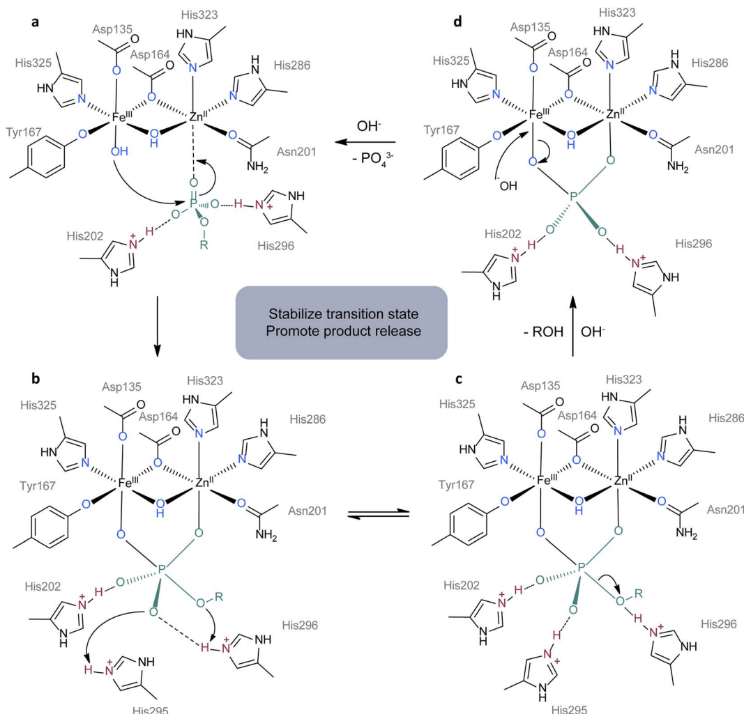
Fig. 4 Proposed mechanism for the hydrolysis of phosphomonoesters by kidney bean purple acid phosphatase. 107 (a) The substance is oriented for attack of Fe III -OH by interactions with Zn II , His202 and His296. (b) RO group in substance attacks protonated His296 and O atom attacks protonated His295. (c) P-O bond breaks with the release of ROH. (d) A hydroxide ion attacks Fe III with the release of the phosphate group to start another cycle of catalysis. The first coordination sphere, second coordination sphere and substrate are colored in blue, red and green. Adapted with permission from ref. 107. Copyright 1996 Academic Press.
