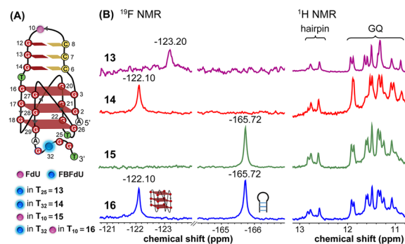
Fig. 4 (A) Schematic representation of the juxtaposed GQ-hairpin structure of the LTR-III + IV region. (B) ^{19}\text{F} NMR and partial ^1\text{H} NMR spectra of ONs 13–16 .
