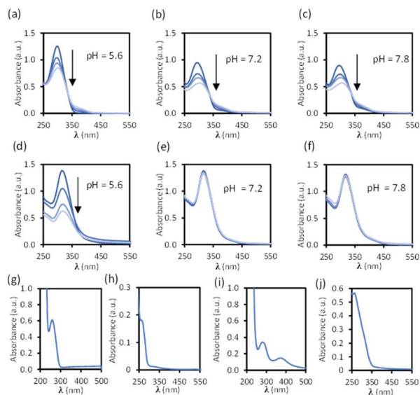
Fig. 5 Stability of cages C1·NO 3 (10 \mu\text{M} , (a–c) 0, 1, 2, 4 days) and C2 (10 \mu\text{M} , (d–f) 0, 1, 2, and 3 days) at different pH values over time in a buffered solution with phosphate (100 \mu\text{M} ) and 1% DMSO. Absorbance spectra of building block components (pH 7.1 buffered solution with phosphate (100 \mu\text{M} ) with 5% DMSO): (g) linker 1 (25 \mu\text{M} ). (h) Pd(II) complex 2·NO 3 (50 \mu\text{M} ). (i) Cavitand 3 (25 \mu\text{M} ). (j) Ligand S2 (20 \mu\text{M} ).
