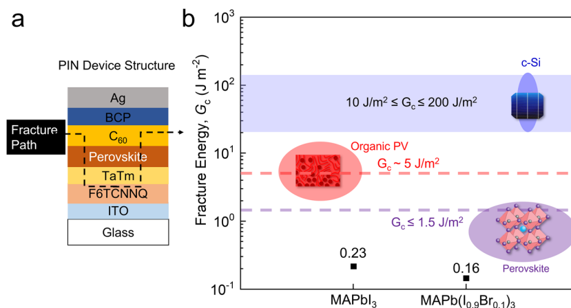
Fig. 2 (a) Device structure and fracture path. (b) The measured average G_c of the p–i–n samples with MAPbI 3 and MAPb(I 0.9 Br 0.1 ) 3 in comparison with the G_c of various PV technologies.
