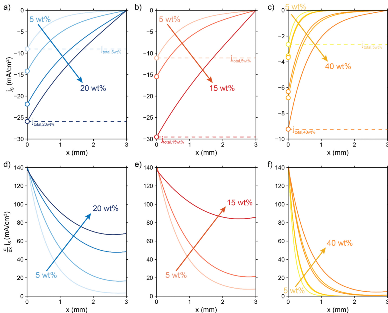
Fig. 7 Modelled local current densities (top figures show j_s , j_L can be found via j_L = j_{s|_x=0} - j_{s|_x} ) and interfacial currents (bottom figures) throughout the electrolyzer channel for (a) and (d) AC, (b) and (e) CB and (c) and (f) GyC slurries. The highest currents and best interfacial current distribution can be achieved in 20 wt% AC and 15 wt% CB suspensions, of which the AC suspension is the most applicable due to higher flowability. The CO 2 reduction reaction is localized near the current collector in all GyC suspensions. All simulations have been run at an R''_{ct} of 10 \Omega cm 2 and an applied potential of −1.5 V versus the membrane (see ESI† for remaining input values).
