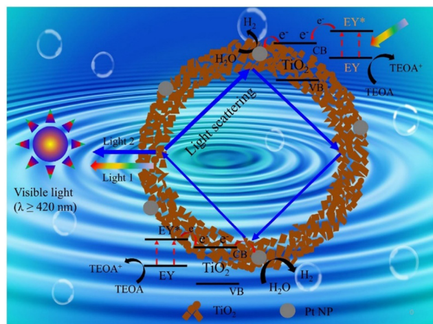
Fig. 13 Mechanism for photocatalytic \text{H}_2 evolution over eosin Y-sensitized C-TiO 2 hollow nanoshells with Mie resonance. Reproduced with permission from ref. 74. Copyright ©2021, Elsevier Ltd.
