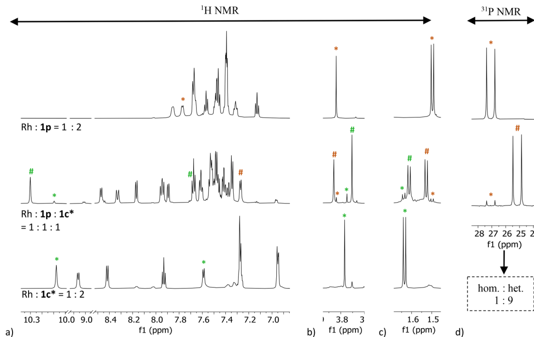
Fig. 4 Stacked ^1\text{H} NMR spectra ( \text{CD}_2\text{Cl}_2 ) of homoleptic and heteroleptic solutions of [\text{Rh}(\text{COD})_2]\text{BF}_4 precursor and 1\text{p} ligand (orange) or/and 1\text{c}^* ligand (green): (a) aromatic region, (b) functional group region, (c) aliphatic region. (d) Stacked ^{31}\text{P} NMR spectra. The homoleptic peaks are indicated by an asterisk (*) and the heteroleptic peaks are indicated by a hash sign (#). Abbreviations: hom.-homoleptic species; het.-heteroleptic species.
