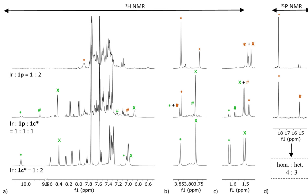
Fig. 5 Stacked ^1\text{H} NMR spectra ( \text{CD}_2\text{Cl}_2 ) of homoleptic and heteroleptic solutions of [\text{Ir}(\text{COD})_2]\text{BARF} precursor and 1\text{p} ligand (orange) or/and 1\text{c}^* ligand (green): (a) aromatic region, (b) functional group region, (c) aliphatic region. (d) Stacked ^{31}\text{P} NMR spectra. The homoleptic peaks are indicated by an asterisk (*), the heteroleptic peaks are indicated by a hash sign (#), the free ligand peaks are indicated by the letter (X). Abbreviations: hom.-homoleptic species; het.-heteroleptic species.
