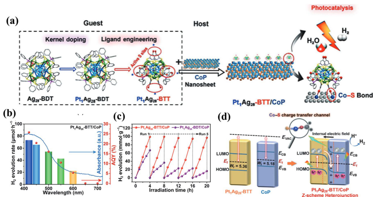
Fig. 7 (a) Schematic of fabrication of the \text{Pt}_1\text{Ag}_{28} -BTT/CoP heterojunction, (b) wavelength dependent hydrogen production and AQY of \text{Pt}_1\text{Ag}_{28} -BTT/CoP, (c) cycling stability of \text{Pt}_1\text{Ag}_{28} -BTT/CoP, and (d) charge transfer mechanism in \text{Pt}_1\text{Ag}_{28} -BTT/CoP. Reproduced with permission from ref. 60. Copyright 2024 Springer.
