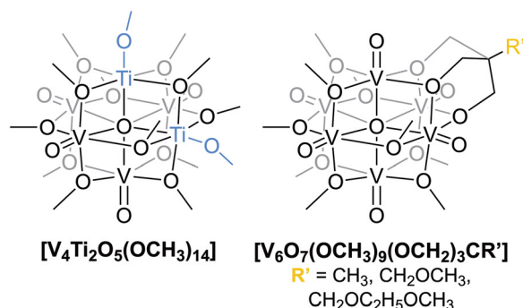
Fig. 1 Examples of inorganic charge-carriers for non-aqueous redox flow batteries.
