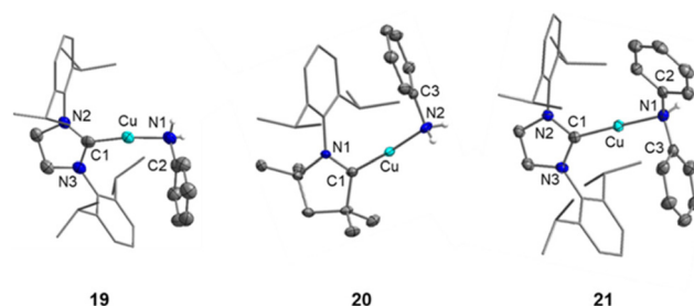
Fig. 5 Molecular structures of the complex cations of [(IDipp)Cu(NH 2 Ph)] + FAP − ( 19 , left), [(cAAC Me )Cu(NH 2 Ph)] + FAP − ( 20 , middle) and [(IDipp)Cu(NHPh 2 )] + FAP − ( 21 , right) in the solid state (ellipsoids set at the 50% probability level; Dipp substituents are shown as wire-and-stick models). Hydrogen atoms except for those of the N atom of the aniline and diphenylamine ligands and a solvent molecule in the crystal structure of 19 are omitted for clarity. Only one of two independent cations in the asymmetric unit of 19 is shown. Selected bond lengths and angles are collected in Table 2 and Fig. S11–S13 in the ESI.†
