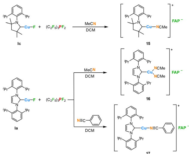
Scheme 3 Synthesis of [(carbene)Cu(LB)] + FAP − complexes 15–17 via fluoride ion abstraction from [(carbene)CuF] using (C_2F_5)_3PF_2 in the presence of N-donor ligands.
