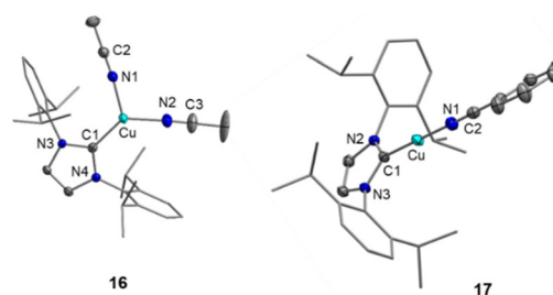
Fig. 4 Molecular structures of the complex cations of [(IDipp)Cu(N≡CMe) 2 ] + FAP − ( 16 ; left) and [(IDipp)Cu(N≡CPh)] + FAP − ( 17 ; right) in the solid state (ellipsoids set at the 50% probability level; Dipp substituents are shown as wire-and-stick models). Hydrogen atoms are omitted for clarity. Selected bond lengths and angles are collected in Table 3 and Fig. S9, S10 in the ESI.†
