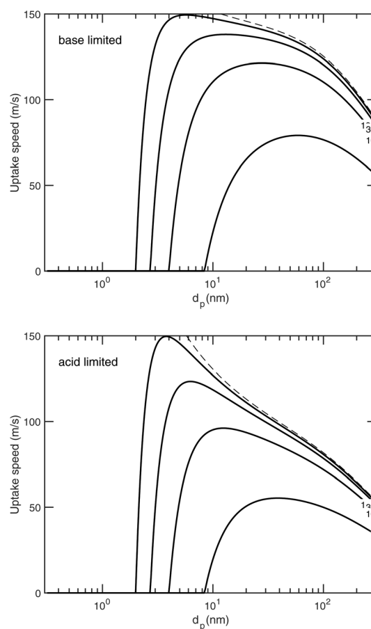
Fig. 17 Uptake speed ( \gamma_{i,p} S_{i,p}^{\text{L}} , black curves) vs. the diameter for flat-surface saturation ratios S^{\circ} = \{3, 10, 30, 100\} and d_{\text{K}10} = 2 \text{ nm} . The S^{\circ} = \infty limit is shown as a dashed curve. (Top) Base-limited ( \text{NH}_3 ) limited uptake assuming no van der Waals enhancement ( A = 0 \text{ joule} ). (Bottom) Acid-limited ( \text{HONO}_2 ) uptake with significant van der Waals enhancement ( A = 6 \times 10^{-20} \text{ joule} ). The collision speed (and thus growth rates) increases rapidly after activation, reaches a maximum and then declines again. The maximum is especially sharp when the van der Waals enhancement is large (i.e. for acid limited conditions in the lower panel).
