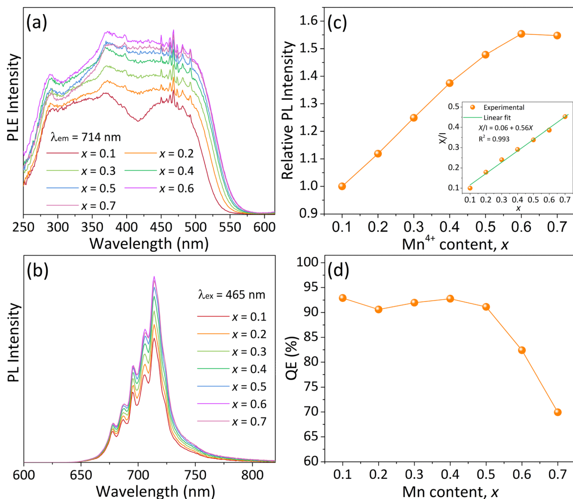
Fig. 6 (a) PLE ( \lambda_{\text{em}} = 714 \text{ nm} ) and (b) PL ( \lambda_{\text{ex}} = 465 \text{ nm} ) spectra of \text{Ca}_{14}\text{Zn}_6\text{Al}_{9.85-2x}\text{Bo}_{0.15}\text{Mn}_x\text{Mg}_{0.35}\text{O}_{35} - 0.42\% \text{ B}_2\text{O}_3 phosphors sintered at 1240^\circ\text{C} for 4 h. Dependence of the integrated PL intensity (c) and QE (d) on the Mn-doping concentration ( x ) of the \text{Ca}_{14}\text{Zn}_6\text{Al}_{9.85-2x}\text{Bo}_{0.15}\text{Mn}_x\text{Mg}_{0.35}\text{O}_{35} - 0.42\% \text{ B}_2\text{O}_3 phosphors.
