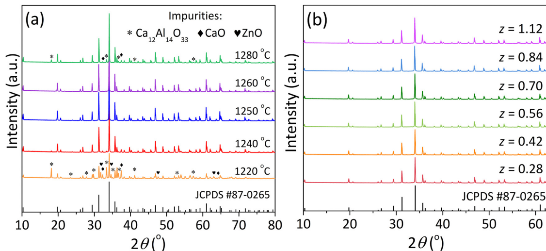
Fig. 1 XRD patterns of (a) \text{Ca}_{14}\text{Zn}_6\text{Al}_{9.8}\text{Mn}_{0.1}\text{Mg}_{0.1}\text{O}_{35} phosphors sintered at various temperatures for 5 h, and (b) \text{Ca}_{14}\text{Zn}_6\text{Al}_{9.8}\text{Mn}_{0.1}\text{Mg}_{0.1}\text{O}_{35} - z \text{ wt\% B}_2\text{O}_3 phosphors sintered at 1240 °C for 4 h. The standard diffraction pattern of \text{Ca}_{14}\text{Zn}_6\text{Al}_{10}\text{O}_{35} from JCPDS (No. 87-0265) is provided at the bottom of the figure.
