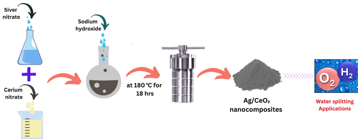
Scheme 1 Preparation of Ag/CeO 2 nanocomposites by a solvothermal method and their application in water splitting.
