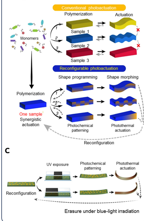
Fig. 5 Artificial muscles with multiple programming-multiple actuation modes (MP-MAM). (a) Conceptual diagram of MP-MAM artificial muscles showing their ability to be programmed, erased, and reprogrammed into entirely different states, enabling multiple actuation modes. (b) Comparison of conventional stimuli-responsive actuators that require distinct programming processes during fabrication for each actuation mode, versus a reconfigurable and reprogrammable artificial muscle capable of multiple shape changes from a single sample through programming, erasing, and reprogramming cycles. (c) Reconfiguration strategy using photochemical and photothermal materials, where pre-memorized states are erased under blue-light irradiation, enabling new configurations. (b) and (c) Reproduced under the terms of the Creative Commons CC BY 4.0 license. 139 (d) Reprogramming magnetic anisotropy in magnetically responsive soft materials via direct laser writing. Localized laser heating melts the polycaprolactone encapsulating NdFeB microparticles, allowing the magnetic particles to realign in the direction of the applied programming magnetic field. Reproduced under the terms of the Creative Commons CC BY 4.0 license. 140 (e) Macroscopically discretionary healing-assembly strategy for reconfigurable artificial muscles. Mechanical assembly and disassembly of building units allow diverse morphing modes, such as “S,” “wave,” “U,” and “heart” shapes, which are achieved through solvent-induced self-healing. Reproduced with permission from WILEY-VCH GmbH, Copyright 2021. 141
