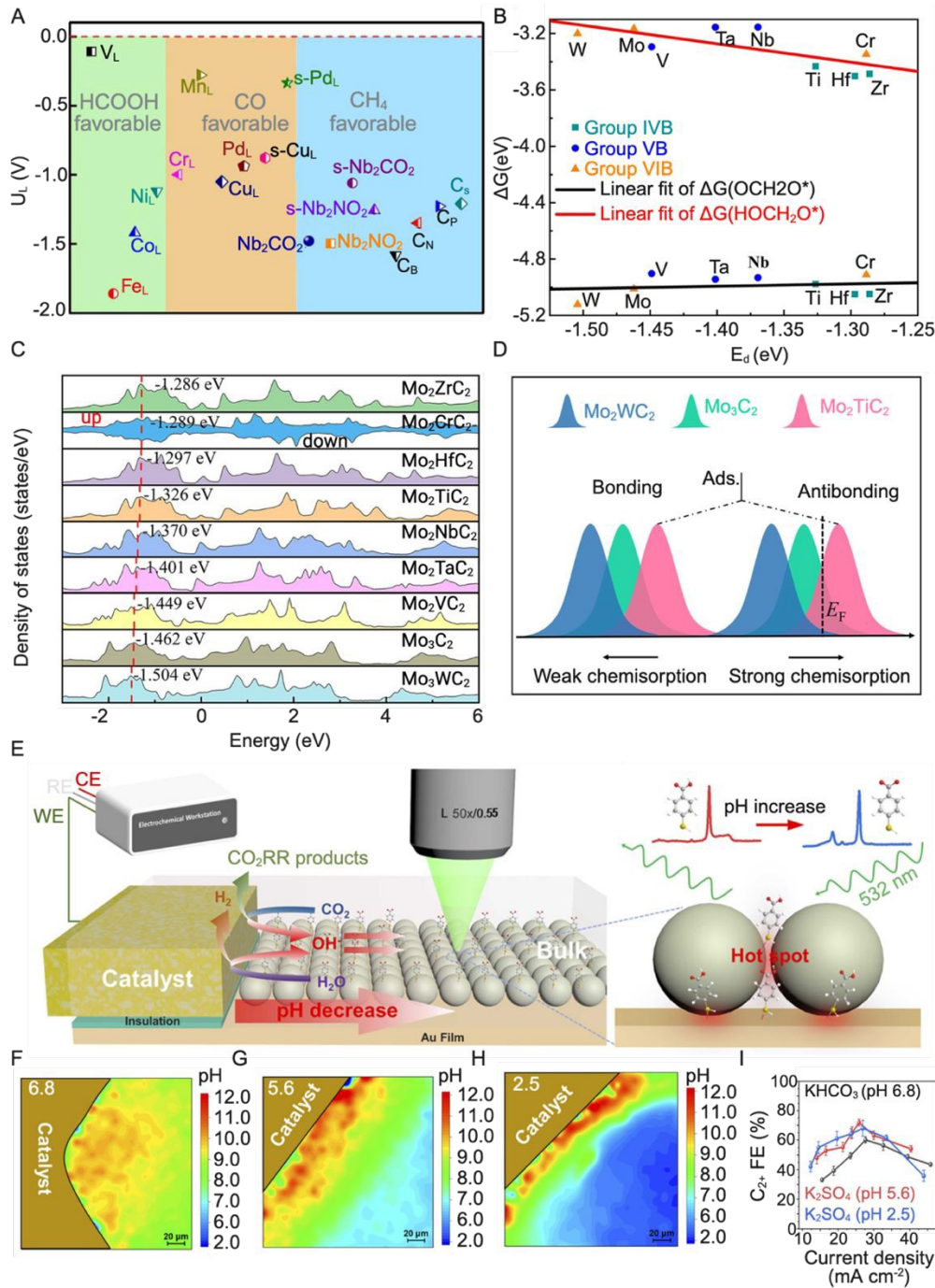
Figure 4. A) Potential limiting UL of \text{NbCO}_2 and modified \text{Nb}_2\text{CO}_2 “Reproduced from reference [74], with permission from Elsevier, Copyright [2021]”. B) Linear relation of adsorption free energy \Delta G(\text{OCH}_2\text{O}^*) and \Delta G(\text{HOCH}_2\text{O}^*) vs. the d-band center E_d . C) Projected density of state plots for the d orbital of surface Mo atoms in MXenes, in which the Fermi level was set to 0, and the calculated d-band centers are denoted by dashed vertical red lines. D) Schematic of the bond formation between the adsorbate (Ads.) and reaction surface of MXenes, represented by \text{Mo}_2\text{WC}_2 , \text{Mo}_3\text{C}_2 , and \text{Mo}_2\text{TiC}_2 . (B-D, “Reproduced from reference [81], with permission from Elsevier, Copyright [2021]” E) Schematic of the L-SERS system for in situ local pH measurement and illustration of pH-sensitive molecules (4-MBA) in the SERS. F–H) Local pH images around the catalyst surface in \text{CO}_2 -saturated electrolyte of (F) \text{KHCO}_3 (pH 6.8), (G) \text{K}_2\text{SO}_4 (pH 5.6), and (H)
