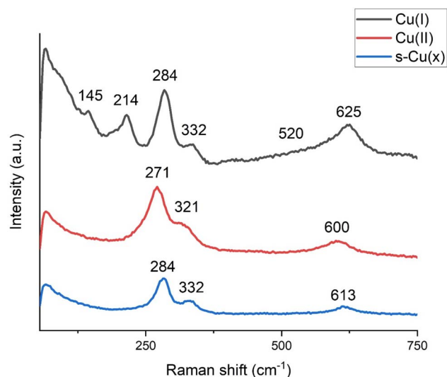
Fig. 5 Raman shift analysis of samples predominantly composed of \text{Cu}_2\text{O} , as Cu(I), CuO, as Cu(II), and laser structured Cu with mixed oxidation states, s-Cu(x).
