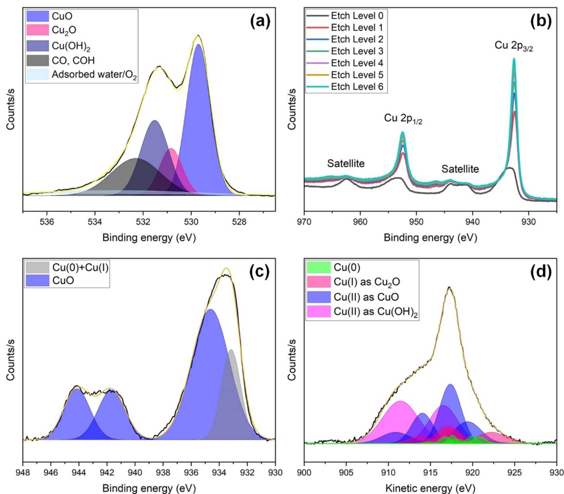
Fig. 6 High resolution XPS spectra of s-Cu(x) prior to ECR studies, showing (a) O 1s, (b) Cu 2p along with a depth profile, (c) Cu 2p_{3/2} , and (d) Cu LMM Auger spectral analysis.
