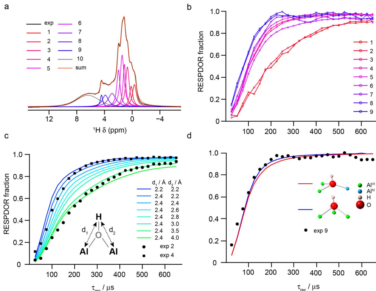
Fig. 10 (a) Decomposition of the 1 H (14.1 T, 40 kHz) DEPTH MAS NMR spectrum of \gamma -Al 2 O 3 dehydrated at 550 °C (blue) into the 10 components used in fits of the RESPDOR spectra. (b) Experimental RESPDOR curves (acquired using R12 3 5 recoupling) plotted as a function of \tau_{\text{rec}} . (c) Overlay of experimental RESPDOR curves for components 2 and 4 with corresponding plots from numerical simulations of a three-spin (H 2 Al) system with varying H–Al distances, as shown. (d) Overlay of the experimental RESPDOR curve for component 9 with corresponding plots from numerical simulations of two four-spin (H 3 Al) systems for \mu_3 aluminols extracted from the structural models above, as shown. In (c) and (d), the 27 Al C Q was 5 MHz and in (c) the angle between the internuclear vectors was also fixed at 60°. For detailed experimental parameters see Section S1 of the ESI†
