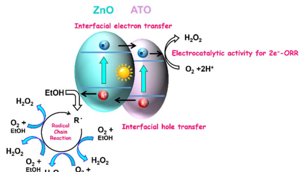
Scheme 1 Schematic description of the action mechanism of ATO-CL/ZnO photocatalysis for the production of \text{H}_2\text{O}_2 from ethanol aqueous solution.
