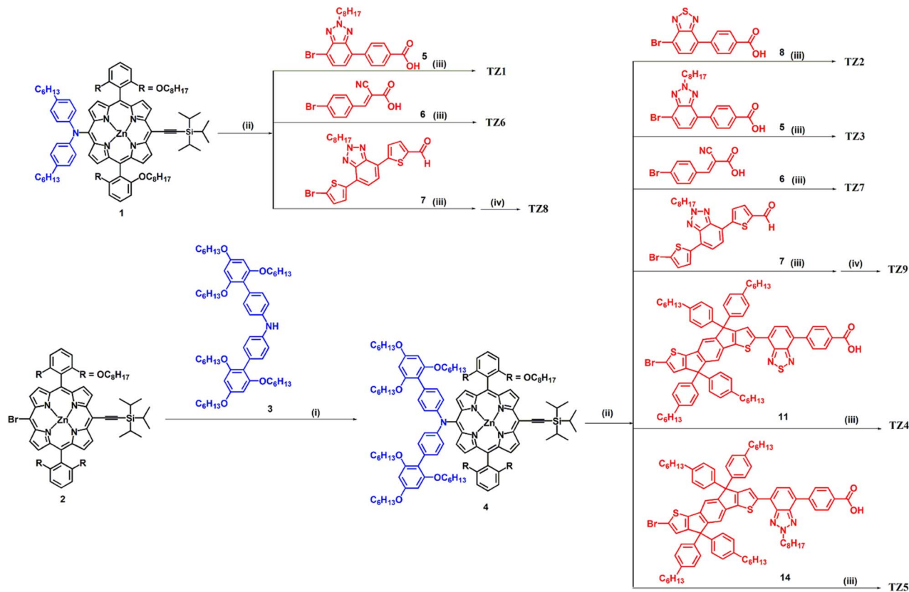
Scheme 1 Synthetic routes of TZ porphyrin dyes. (i) Pd(OAc) 2 , NaOtBu, P(tBu) 3 , toluene. (ii) tetra- n -Butylammonium fluoride (TBAF), THF. (iii) Pd 2 (dba) 3 , AsPh 3 , Et 3 N, THF. (iv) 2-cyanoacetic acid, piperidine, CHCl 3 .
