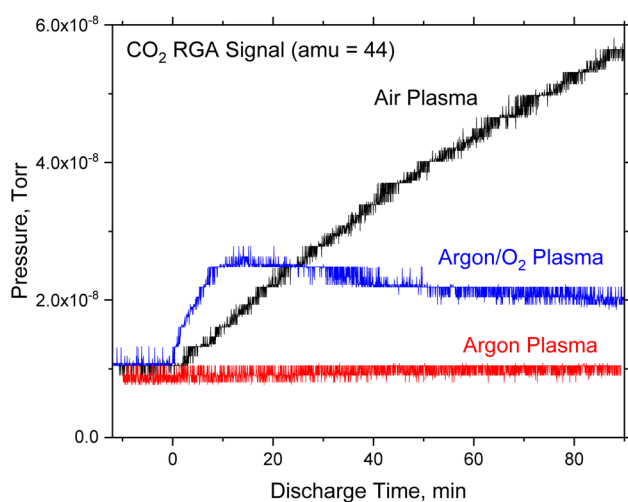
Fig. 5 The comparison of RGA CO_2 signals ( amu = 44 ) under argon, 50% oxygen (balanced by Ar) and air plasmas with the presence of CaCO_3 powders.
