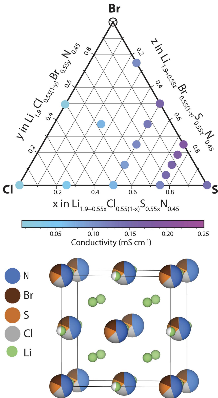
Fig. 6 Investigating conductivities in the \text{Li}_{1.9+0.55y}\text{Cl}_{0.55(1-y-z)}\text{S}_{0.55y}\text{Br}_{0.55z}\text{N}_{0.45} ( 0 < y, z < 1 ) space. Quasi-ternary phase diagram with the \text{Li}_{1.9}\text{Cl}_{0.55}\text{N}_{0.45} , \text{Li}_{1.9}\text{Br}_{0.55}\text{N}_{0.45} and the \text{Li}_{2.45}\text{S}_{0.55}\text{N}_{0.45} compositions at its vertices. The circles represent the phase-compositions that were synthesized as part of this work. Coloured circles signify pure-phase antiperovskite-like products. Hollow circles signify no pure-phase antiperovskite-like phase product. The colors correspond to experimentally measured ionic conductivities at 22 °C. A schematic unit cell of the phase space investigated is also shown.
