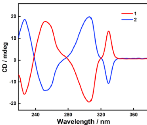
Scheme 47 (Left) Chemical structures of the ligands and Ln complexes (1/2), adapted from ref. 105. (Right) CD spectra of 1 (red) and 2 (blue) in \text{CH}_2\text{Cl}_2 , reproduced from ref. 105 with permission from the Royal Society of Chemistry, copyright [2022]. 105
