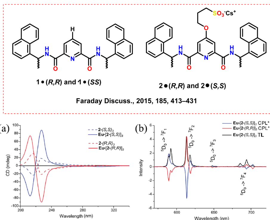
Scheme 23 (Above) Chemical structures of the ligands (2(R,R) and 2(S,S)). 67 (Below) (a) Overlaid CD spectra from 2•(S,S) 3 , 2•(R,R) 3 (dashed) at 1 \times 10^{-5} M and \text{Eu} \cdot [2 \cdot (R,R)]_3 , \text{Eu} \cdot [2 \cdot (S,S)]_3 (solid) at 3.3 \times 10^{-6} M in water at 24 °C (b) CPL and total luminescence (TL) spectra recorded for \text{Eu} \cdot [2 \cdot (R,R)]_3 and \text{Eu} \cdot [2 \cdot (S,S)]_3 in water. Reproduced from ref. 67 with permission from the Royal Society of Chemistry, copyright [2015]. 67
